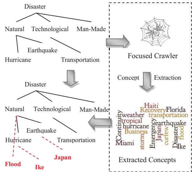
Figure 3. Iterative taxonomy generation
