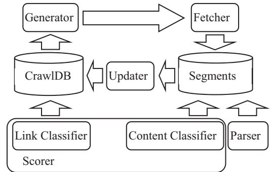
Figure 6. Architecture of the focused crawler.
